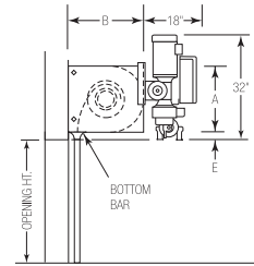
GEARHEAD VERTICAL MOTOR
