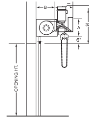
GEARHEAD VERTICAL MOTOR
