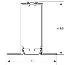
BOTTOM BAR DETAIL
