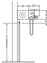
BELT DRIVE MOTOR
