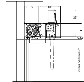
FMF GEARHEAD VERTICAL MOTOR
