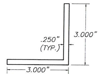
(E) 3"x3"x1/4" INSIDE MOUNT ANGLE 6061-T6 ALUMINUM ALLOY SCALE: 3/8" = 1"
