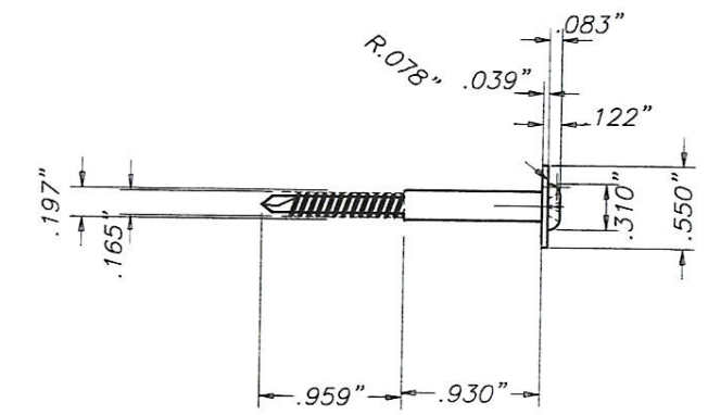
(C) RETAIN SCREW (1 EVERY OTHER SLAT INCLUDING BASE SLAT AND SHALL BE INSTALLED W/A 0.576" MIN. SLIP AS SHOWN ON SECTIONS) AISI/SAE 304 SERIES STAINLESS STEEL SCALE: 3/4" = 1"
