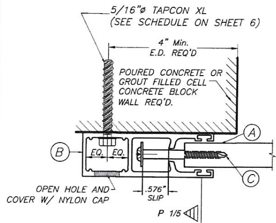
SECTION P-P (1): WALL MOUNT
