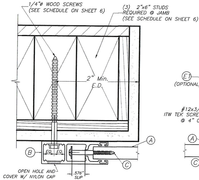
SECTION P-P (1): WALL MOUNT
