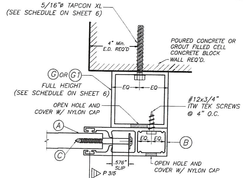
SECTION P-P (3): BUILD-OUT
