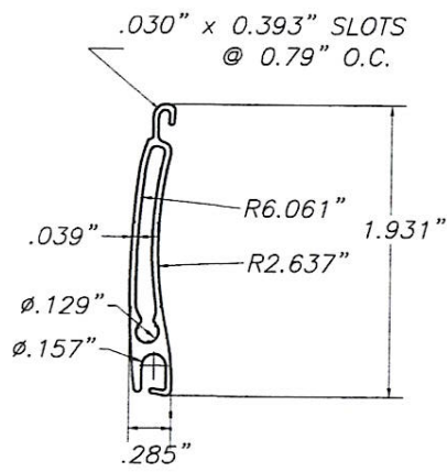
(A) SLAT 6063-T6 ALUMINUM ALLOY SCALE: 3/4" = 1"
