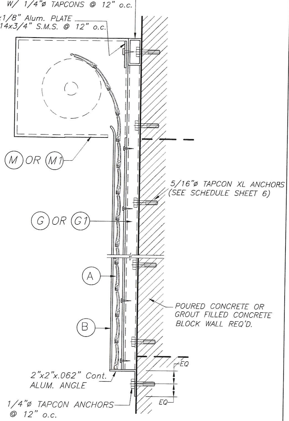
SECTION P-P (3)
